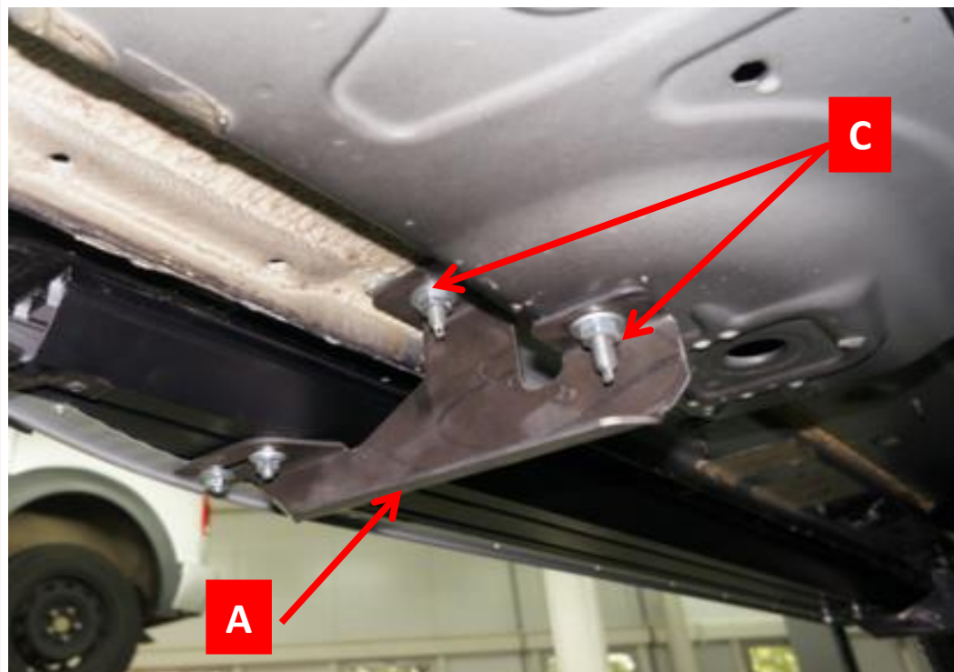
FRONT BRACKET
